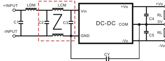
(EMC 推荐电路图 3)
